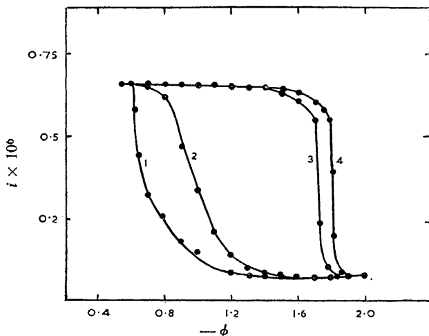
FIG. 4.—Current-voltage curves of 10^{-3}\text{N K}_3\text{Fe}(\text{CN})_6 + x[(\text{C}_4\text{H}_9)_4\text{N}]_2\text{SO}_4 solutions. 1, x = 0 ; 2, x = 10^{-5}\text{N} ; 3, x = 5 \times 10^{-5}\text{N} ; 4, x = 10^{-4}\text{N} .
