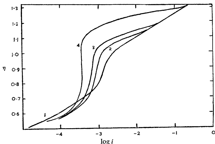
FIG. 11.—Hydrogen overvoltage on mercury in 2\text{N HCl} + 2\text{N KI} + x\text{N}(\text{C}_4\text{H}_9)_4\text{Br} solutions.
