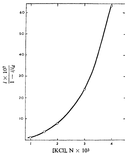
FIG. 3.—Dependence of the current strength at the minimum of the current-voltage curve in \text{K}_3\text{Fe}(\text{CN})_6 + KCl solutions on the concentration of KCl; current corrected for concentration polarization.
