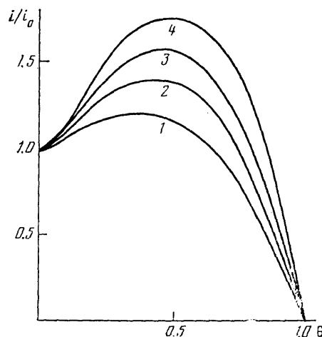
Figure 7. Dependence of the current for the electroreduction of doubly-charged cations on the degree of coverage of the electrode surface by inactive singly-charged organic anions. 52,53
