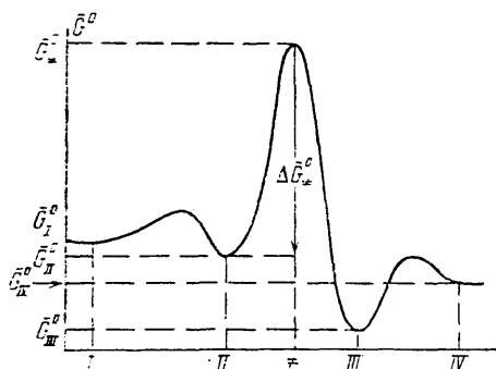
Figure 1. Diagram representing the change in the standard electrochemical free energy of a system \bar{G}^0 along the reaction path.
