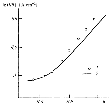
Figure 8. Dependence of the current for the electroreduction of the cationic complex \text{cis-Cr(en)(NCS)}^+ on the degree of coverage of the mercury electrode surface: 1) experimental points, 2) results of the calculation using Eqns. (50) and (51).
