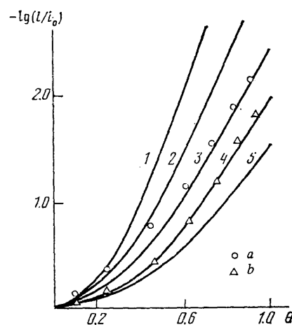
Figure 3. Inhibition of the electroreduction of cadmium cations in the presence of t-butylamine (a) and t-butyl alcohol (b); the continuous lines give the results of the calculation with the following fixed values of the parameters: \alpha = 0.5 , \delta = 3 Å, \Gamma_{\infty} = 1.5 \times 10^{14} cm -2 , x_0 = 1.5 Å, z = 2 , z_0 = 1 , \epsilon_{pl} = 8 and different x_a = 0.5, 1.0, 1.5, 2.0 , and 2.5 Å (curves 1–5 respectively).
