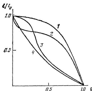
Figure 6. Dependence of the current for the electroreduction of doubly-charged cations on the degree of coverage \theta under the conditions of the combined adsorption of dipolar molecules of two kinds 57 with the following values of the dipole moments: 1) \mu_1 = \mu_2 = 1 ; 2) \mu_1 = 1, \mu_2 = -1 ; 3) \mu_1 = -1, \mu_2 = 1 ; 4) \mu_1 = \mu_2 = -1 CGSE unit.
