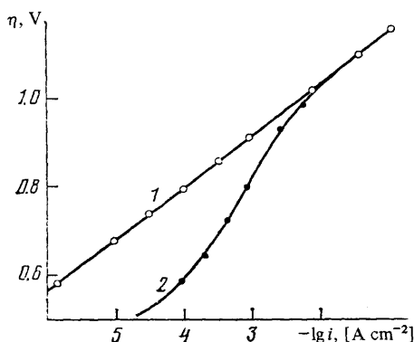
Figure 2. Polarisation curves for the discharge of hydrogen ions on mercury from aqueous solutions of 1 M HCl + 2 M KCl (1) and 1 M HCl + 2 M KI (2); continuous lines—result of the theoretical calculation. 46,47
