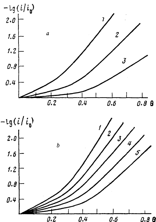
Figure 4. Theoretical relationships 48,49 characterising the effect of the inhibition of an electrode process by adsorbed dipolar molecules (the reduction of doubly-charged cations on mercury in the presence of molecules with \mu = -1.6 \text{ D} , oriented mainly with the positive pole towards the electrode): a) influence of the orientation of the dipole relative to the reactant ion; b) influence of the orientation of the dipole relative to the electrode surface.
